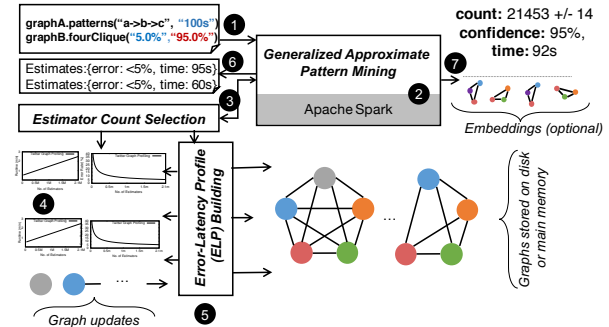
Figure 3: ASAP architecture
